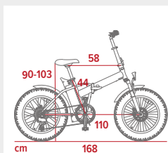
E-bike dimensions
