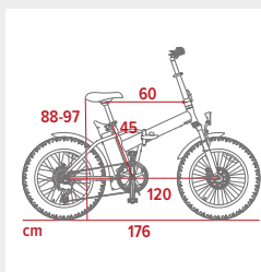
E-bike dimensions
