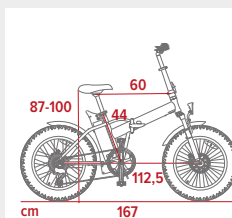
E-bike dimensions
