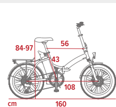
E-bike dimensions
