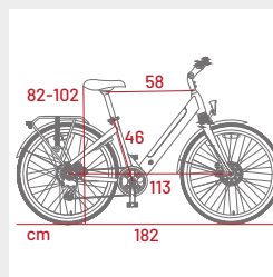
E-bike dimensions
